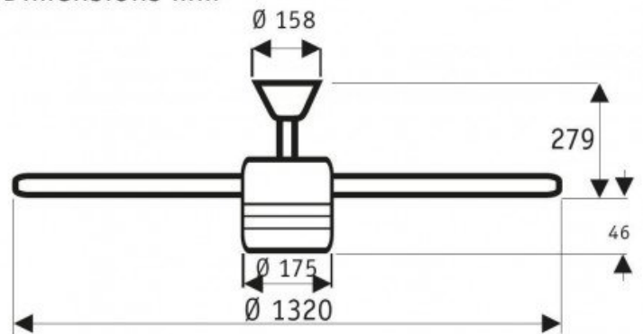
Dimensions mm
