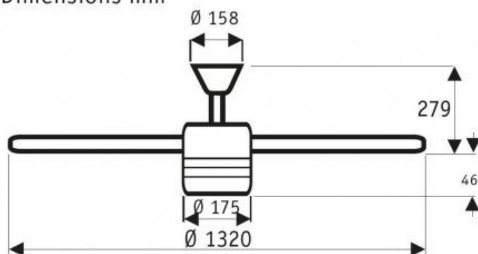
Dimensions mm
